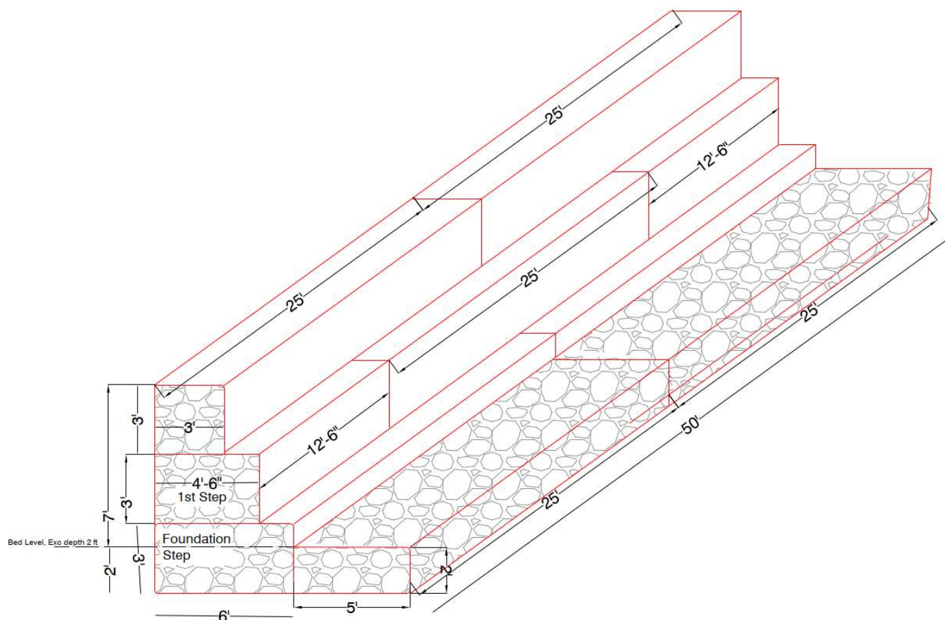
Isometric View
