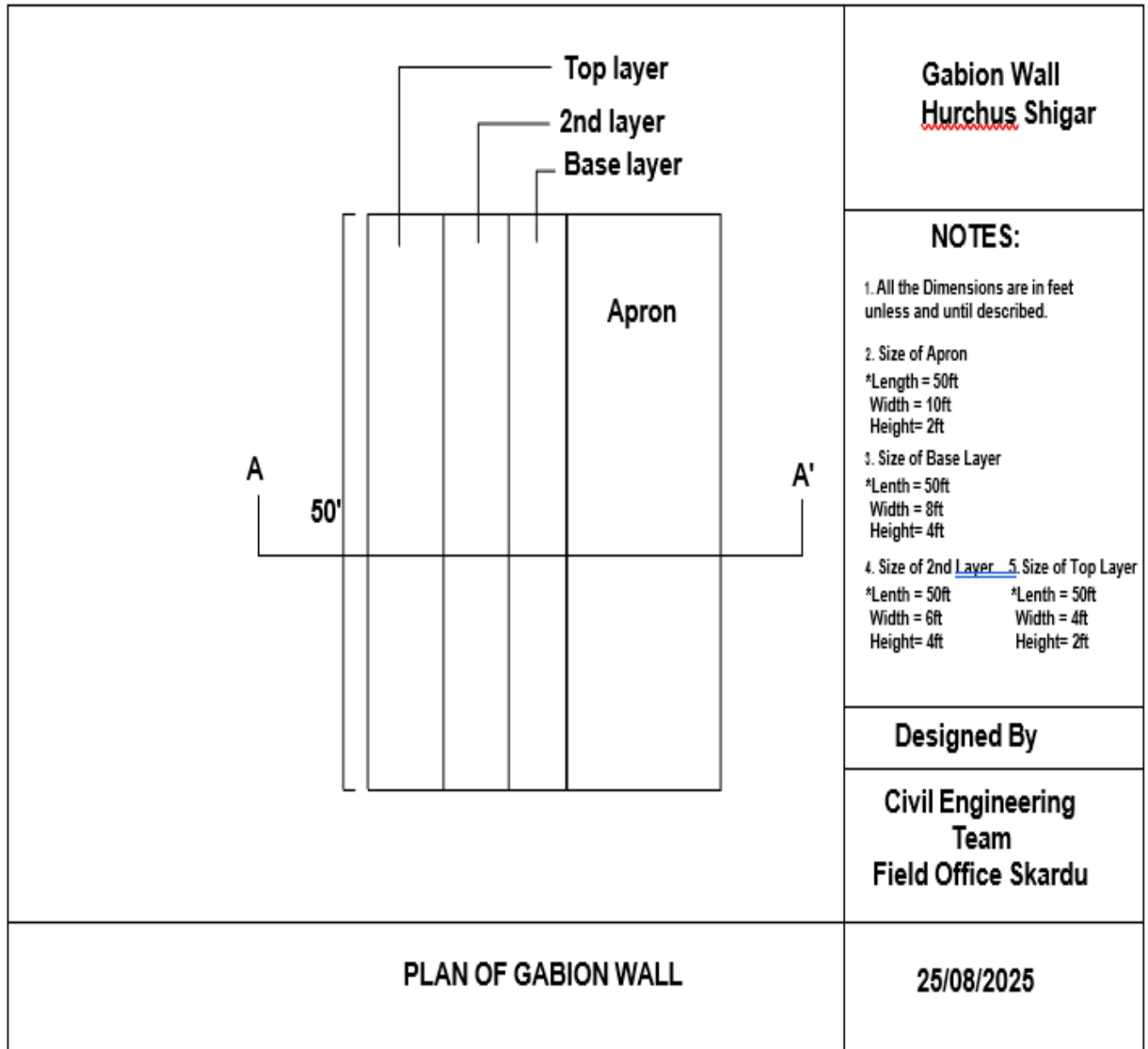
Drawing: Construction of Gabion Protection Bund.
