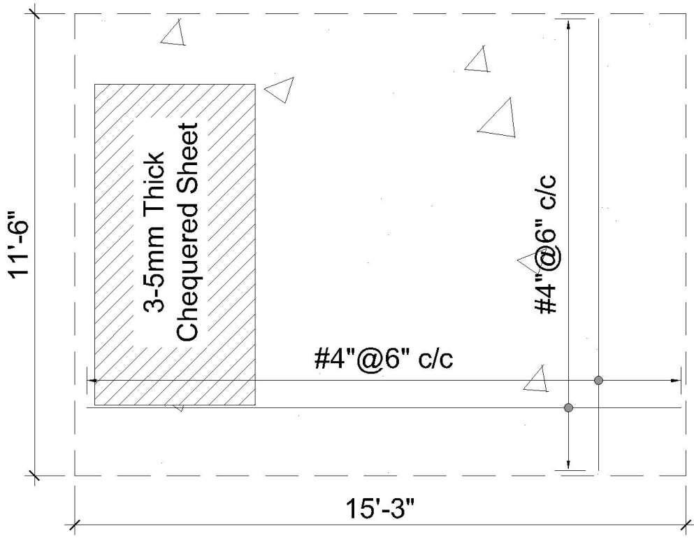
Top Slab
